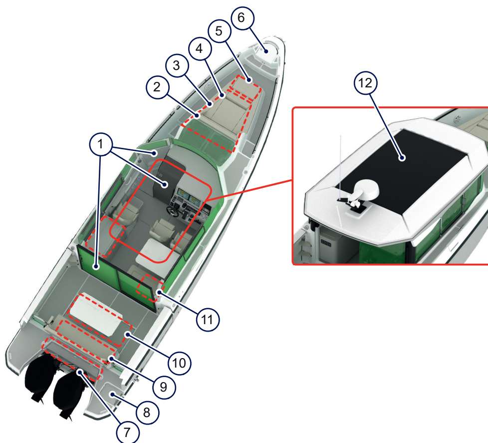
Figur 4.27 - Luckor
